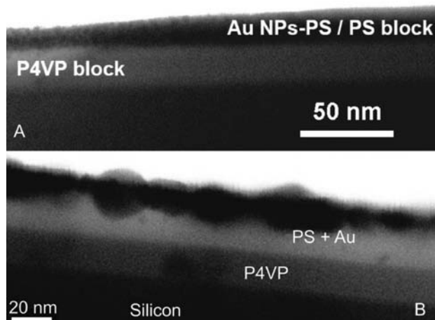
Figure 2. Cross-sectional HAADF-STEM images of P4VP- b -PS brushes infiltrated with PS-covered Au NP after annealing with CH 2 Cl 2 vapor: (a) \Sigma_{PS} = 1.79 chains nm -2 and (b) \Sigma_{PS} = 0.95 chains nm -2 . The intensity of the images was inverted for improved visibility. The gradient in brightness, most noticeable in (a), arises from the variation in sample thickness, due to sample preparation. Layer thicknesses of 16 nm P4VP and 20 nm PS in Figure 2b are in good agreement with original layer thicknesses of 13 and 19 nm, respectively.
